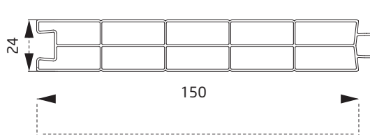
PTS2360BY 24 mm lambri 24 mm paneling
