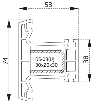
PSY4765BY Sineklikli Kasa Profili Frame Fly Screen Profile
