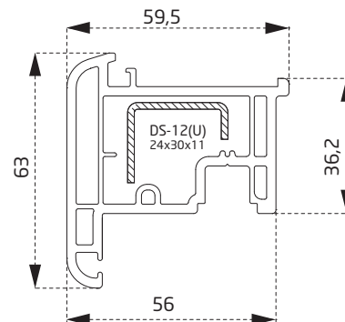
PVN1360BY Stump Profili Stump Profile
