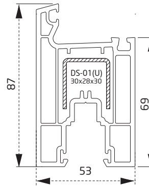
PSY4665BY Fix Kasa Profili Fix Frame Profile
