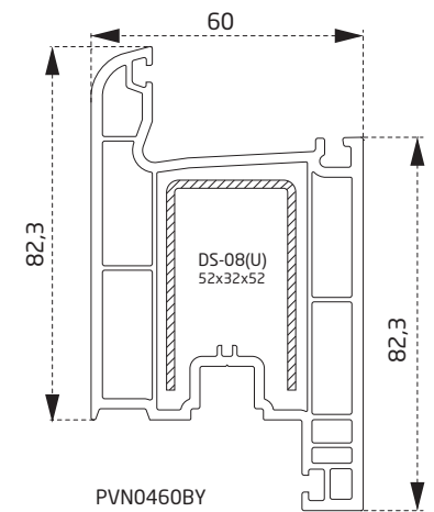
PVN0460BY Kapı Profili Opening Door Profile
