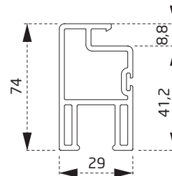
PSY4765BY Kanat Profili Sash Profile
