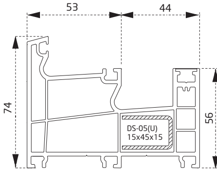
PSY0165BY Kasa Profili Frame Profile
