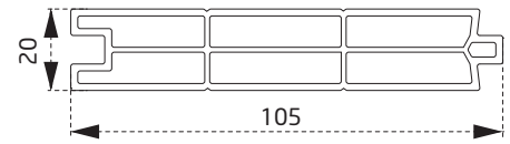
PTS2260BY 20 mm lambri 20 mm paneling
