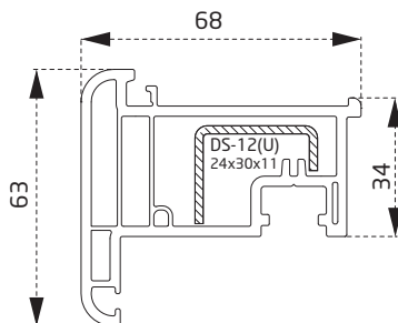
PDR1360BY Stump Profili Stump Profile
