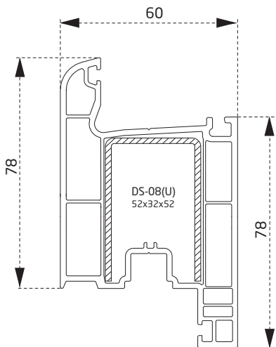
PRVNEC04B Kapı Profili Opening Door Profile
