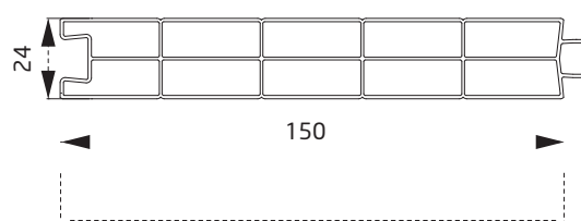
PTS2360BY 24 mm lambri 24 mm paneling
