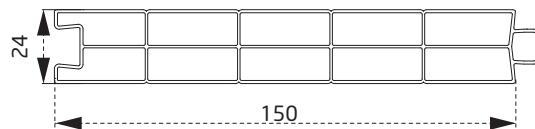
PTS2360BY 24 mm lambri 24 mm paneling
