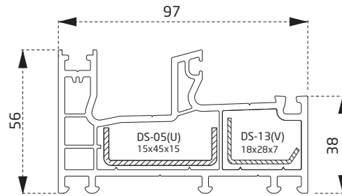
PSY4665BY Fix Kasa Profili Fix Frame Profile
